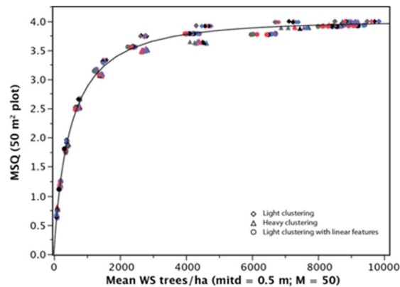
Figure 4. Comparison of simulated WS and MSQ survey outcomes. Spatial patterns correspond to those illustrated in Figures 1b to 1d. Stands with a random spatial pattern were not included.
