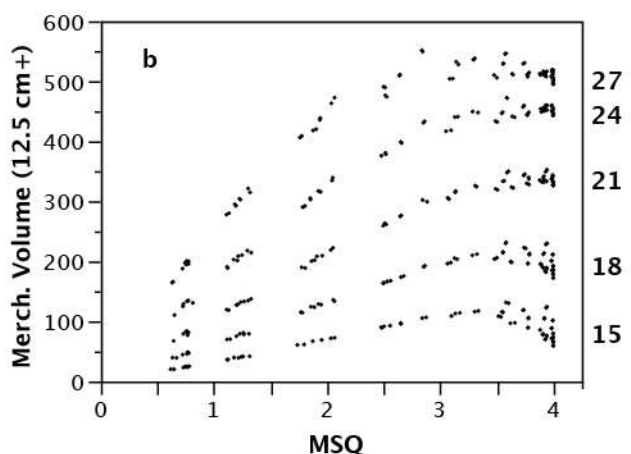
Figure 3b. Impact of merchantability limits on PMV curve shape. For the lowest site indices, PMV value (merchantable as opposed to total volume) start to decline at the highest MSQ values. This effect results from a significant proportion of trees falling below the merchantable dbh limit. This trend is exacerbated for stands with the highest stand densities, which correspondingly experience the highest risk of merchantable yield declines. This effect is largely absent for site indices 24 and 27.
