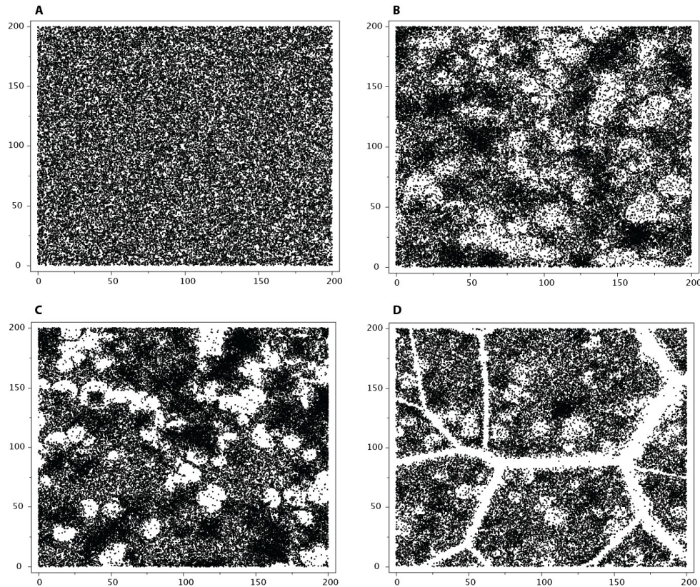
Figure 1. Stem maps illustrating the 4 simulated spatial patterns used to generate deciduous MSQ models, in this case for stands with 12,800 suckers per hectare. The scale is in metres, and each dot represents a tree location. The pattern in (A) represents a completely random distribution, (B) and (C) represent increasing levels of clumping, and (D) builds upon (B) with the addition of linear features such as wet draws and harvest trails that could impact on stocking levels.
