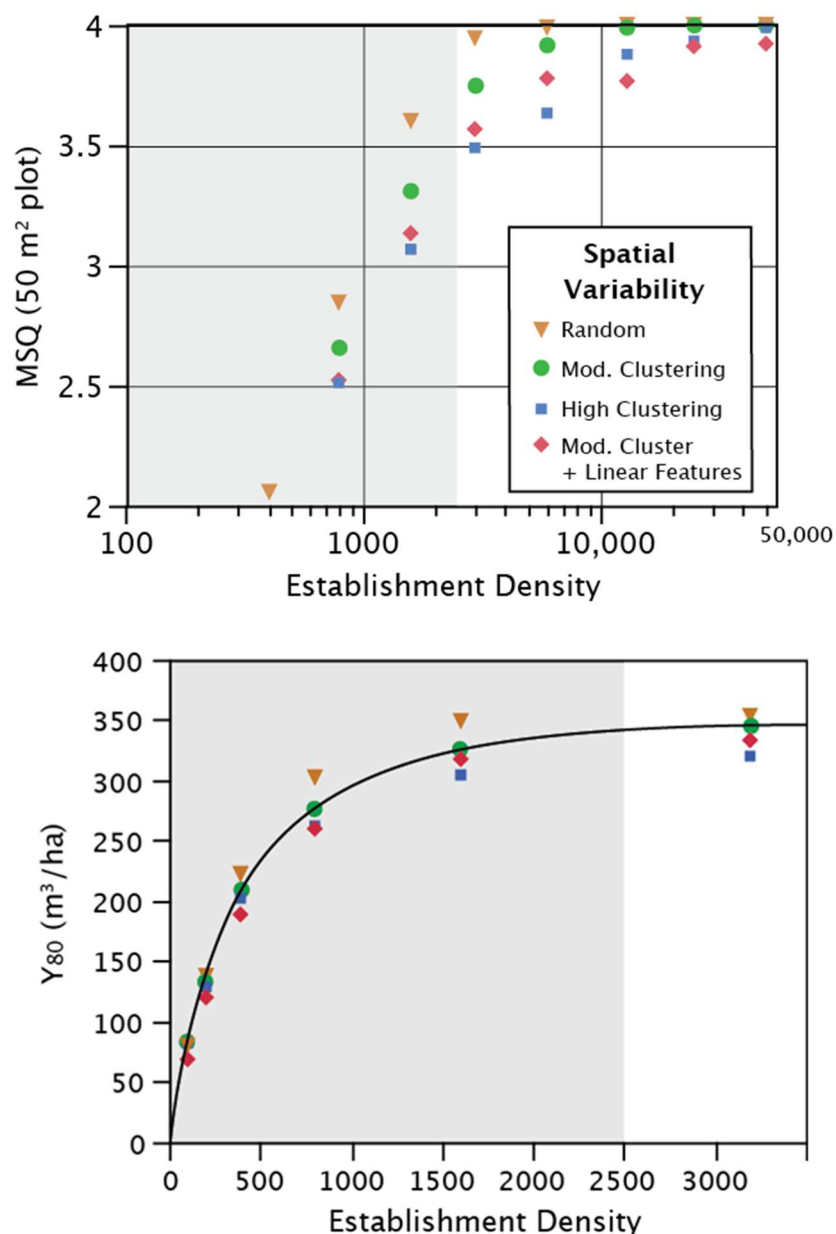
Figure 8. Comparison of total stand densities as modeled in TASS with MSQ values (top) and merchantable yield for SI50 = 21 (bottom). The relationships between these measures vary with spatial pattern, represented here using the four patterns from Figure 1. The grey zones represent stand densities for which there was no calibration data available for TASS. Note that critical MDQ threshold values for stocking acceptability range from 2.5 to 3.25, depending on SI (from Figure 3c). Note also the equivalent total stand densities in the field will be higher when the presence of trees with unacceptable levels of vigour and damage are included in the tally.
