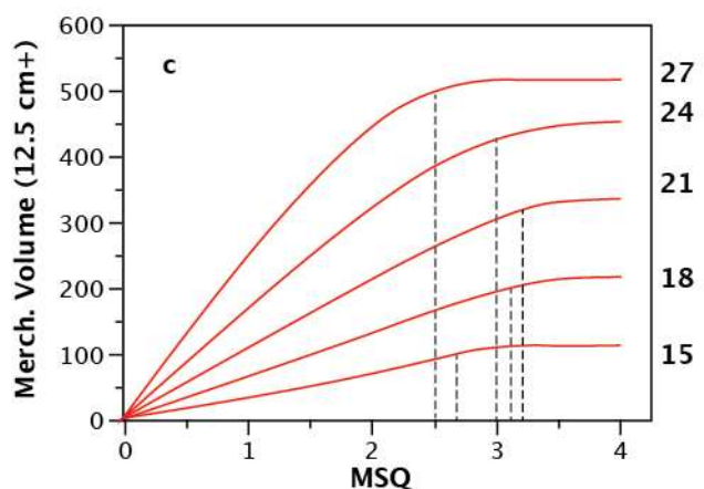
Figure 3c. Impact of site index and merchantability limits on TMV thresholds. PMV curves have been fit to the data points from 3b. Any stands established at densities above 10,000 trees/ha for SI's 15 and 18 have been ignored to avoid the merch volume drop-off associated with high MSQ values shown in Figure 3b above. Relative to relationships for SI = 21, SI's 24 and 27 experienced lower TMV values as a result of improve growing space occupancy by fewer trees, while SI's 15 and 18 experience lower TMV's as a result of the merchantable yield reductions associated with high establishment densities (which are strongly correlated to high MSQ's).
