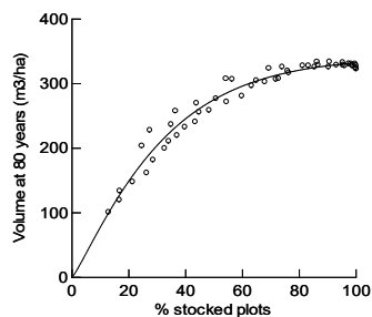
Figure 4. Relationship between merchantable volume/ha at age 80 and percent stocked plots at survey. Solid line is fitted regression.
