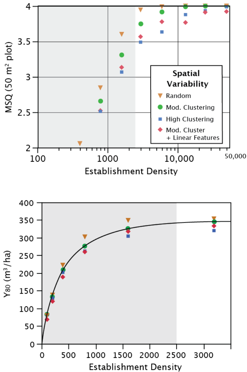
Figure 8. Comparison of total stand densities as modeled in TASS with MSQ values (top) and merchantable yield for SI_{50} = 21 (bottom). The relationships between these measures vary with spatial pattern, represented here using the four patterns from Figure 1. The grey zones represent stand densities for which there was no calibration data available for TASS. Note that critical MSQ threshold values for stocking acceptability range from 2.5 to 3.25, depending on SI (from Figure 3c). Note also that equivalent total stand densities in the field will be higher when the presence of trees with unacceptable levels of vigour and damage are included in the tally.
