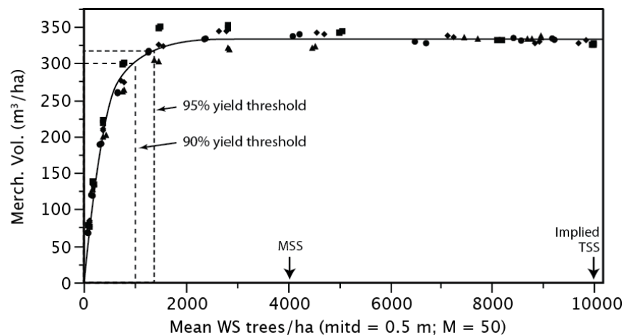
Figure 5. Predicted yield by WS stocking for current stocking standards (MSS = minimum WS). Based on this relationship, it appears that a 0.95 volume threshold would be achieved at approximately 1400 WS trees/ha. This is roughly equivalent to 2000 to 3000 countable/acceptable trees/ha depending on tree spatial pattern.
