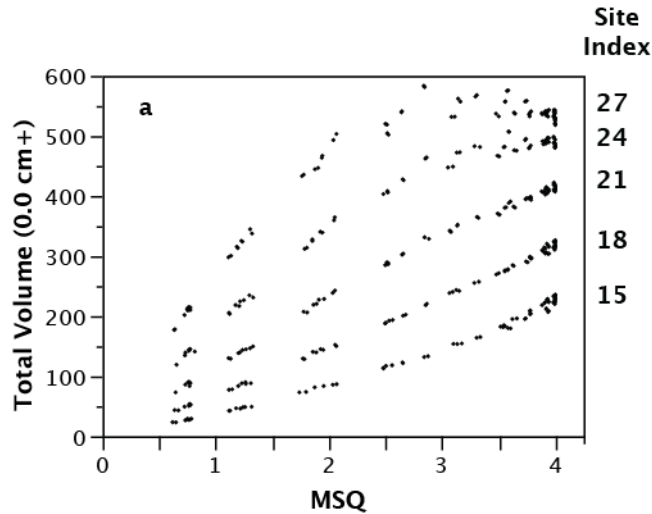
Figure 3a. Impact of growth rates on PMV curve shape, based on total volume. At very high site indices (e.g. SI = 27 m), it takes fewer trees than at lower site indices to maximize use of available growing space. For SI = 21 and lower, total yield continues to increase right up to MSQ = 4, but yield plateaus at lower MSQ's for the higher SI's.
